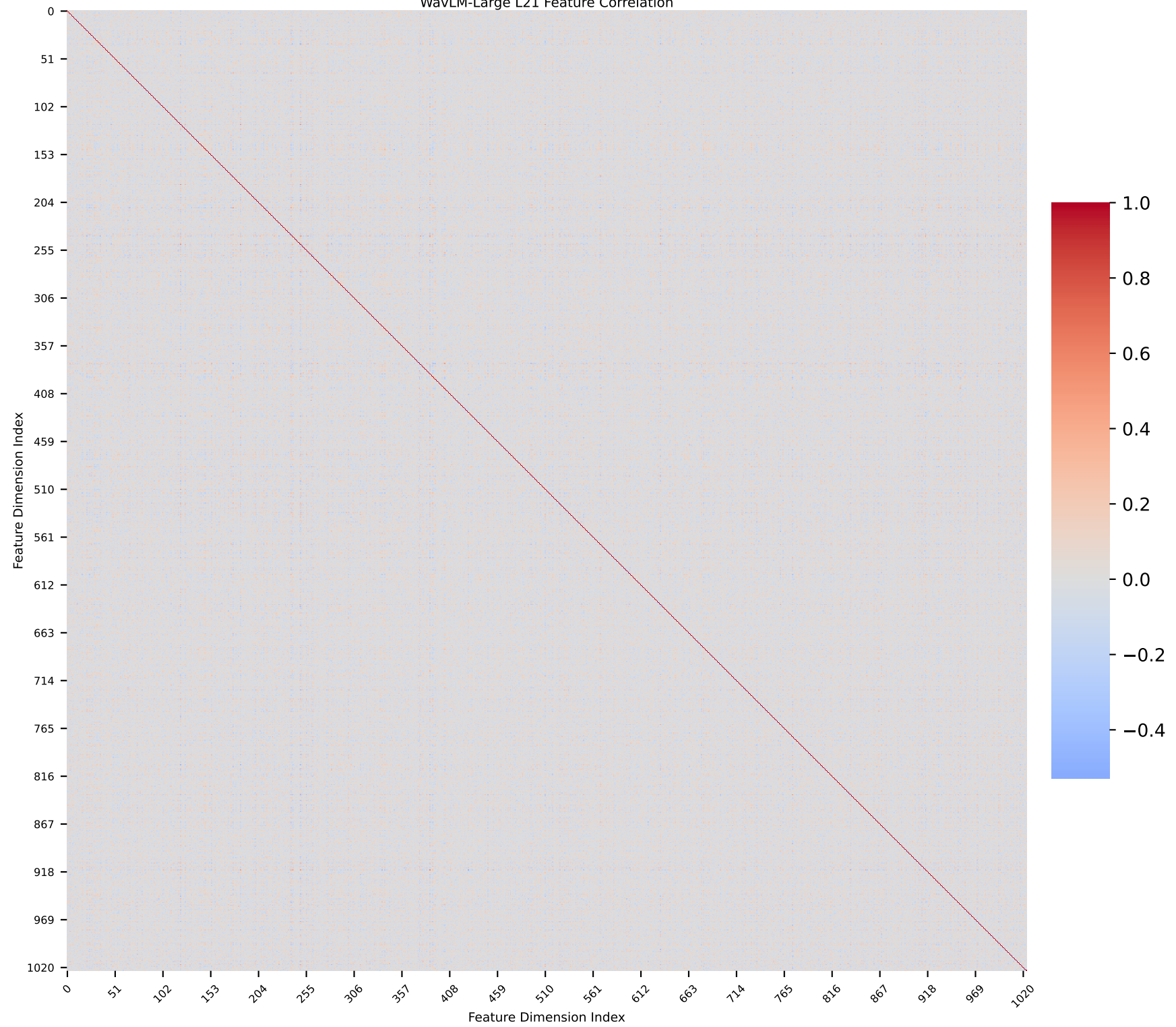
WavLM-Large L21 Feature Correlation
